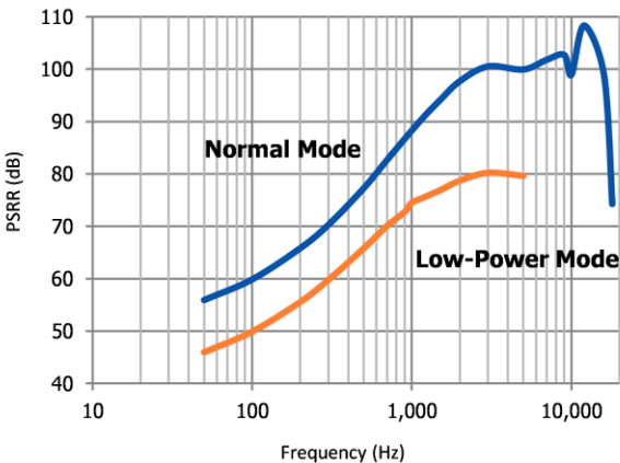
Figure 12: Typical PSRR
