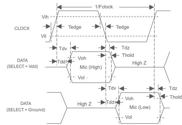
Figure 1: Timing Diagram
