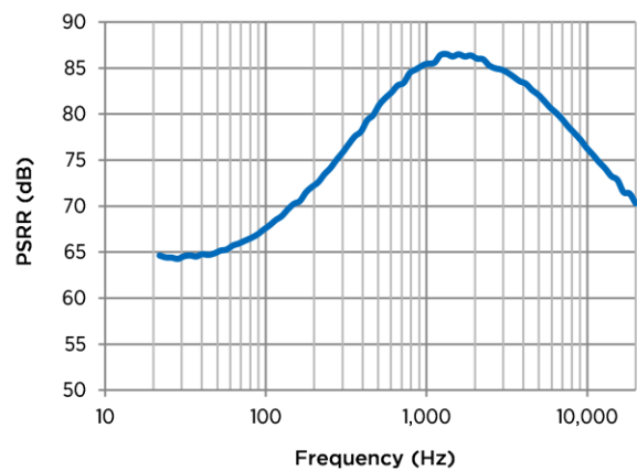
Figure 10: Typical PSRR
