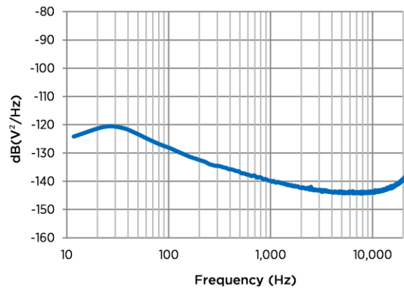
Figure 10: Typical PSRR
