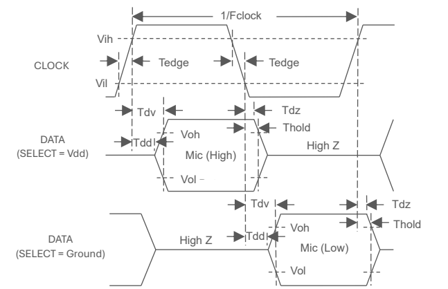
Figure 1: Timing Diagram
