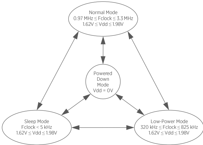
Figure 3: State Diagram
