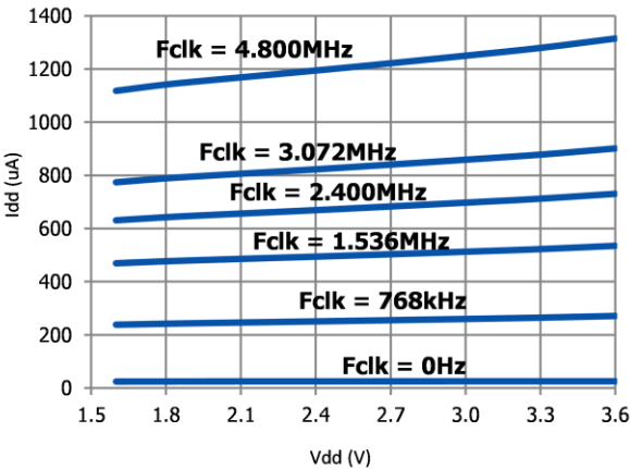
Figure 11: Typical Idd vs Vdd
