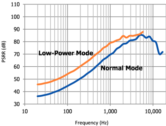
Figure 13: Typical PSRR
